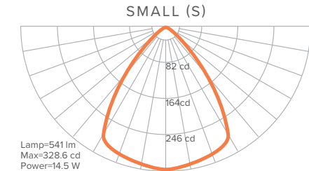
LUMINOUS INTENSITY DISTRIBUTION
