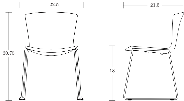
Sled Base Side / SLS
