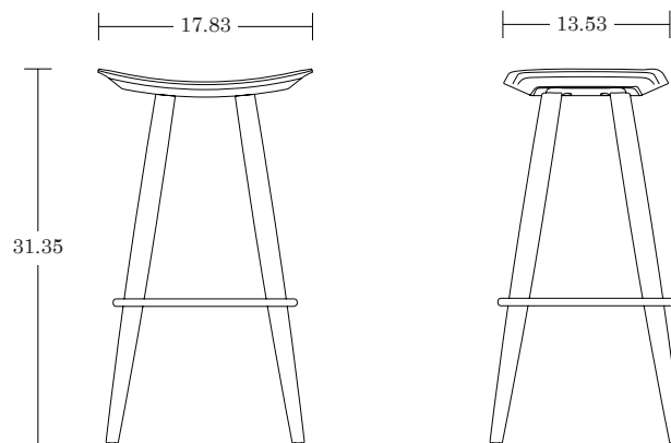
Upholstered Seat / OMBWU
